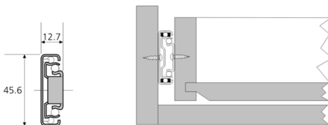
Installation Diagram
