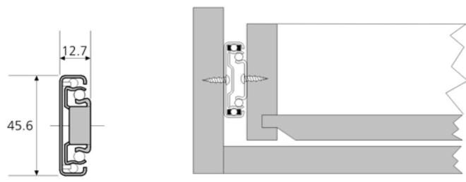
Installation Diagram
